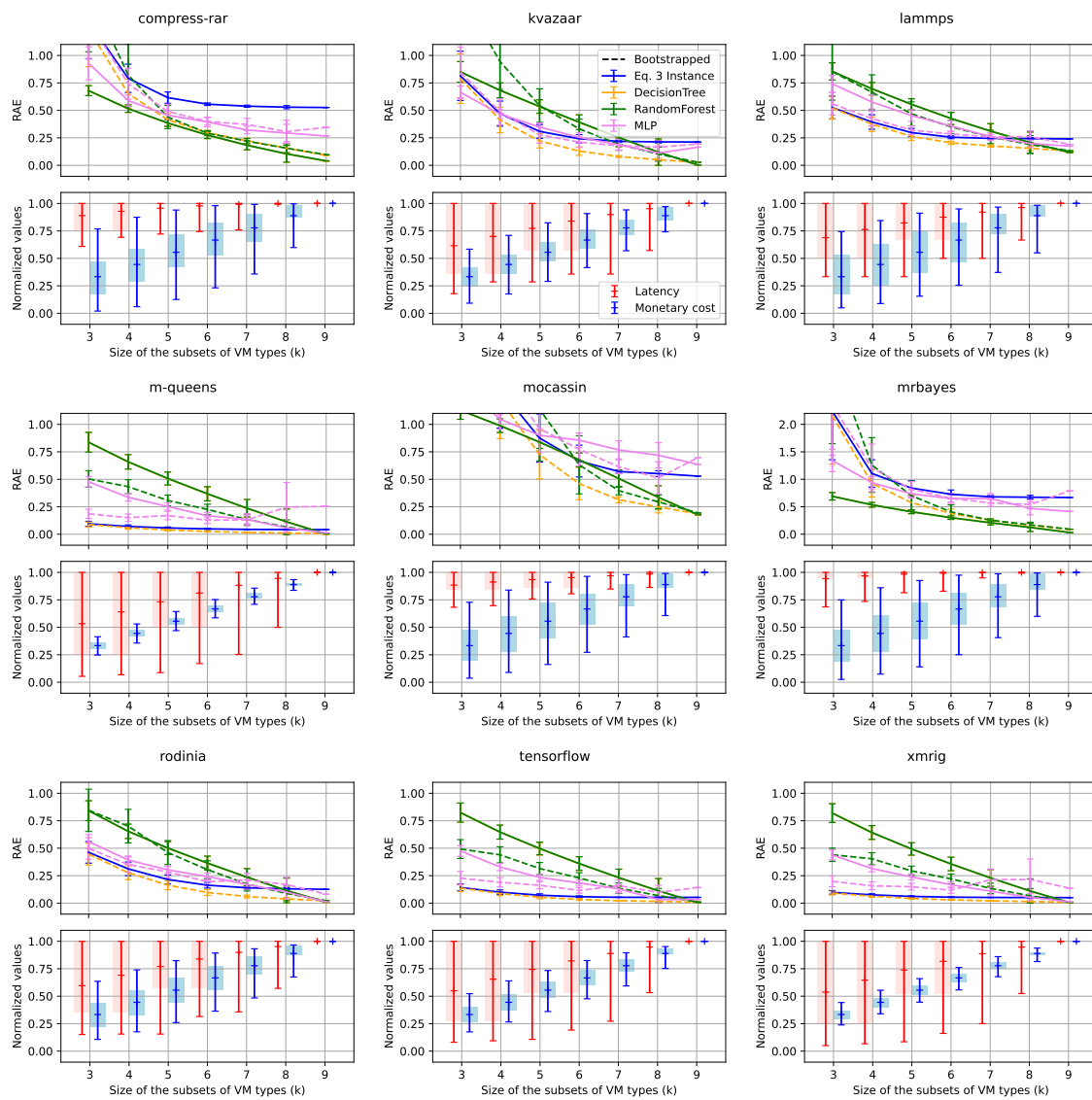
Fig. 2. Results with the C7a family for all benchmark applications
